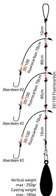
Montage Surfcasting Classic
