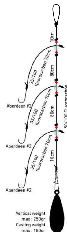
Montage Surfcasting Pro
