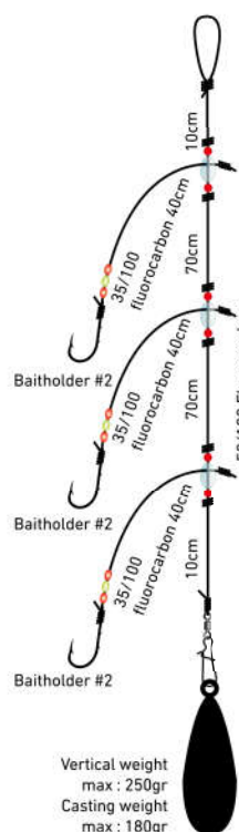
Montage Surfcasting Essential Classic
