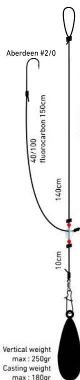
Montage Bar Surfcasting
